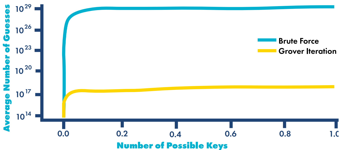
Figure 5: Speedup of Grover Iteration vs Brute Force
